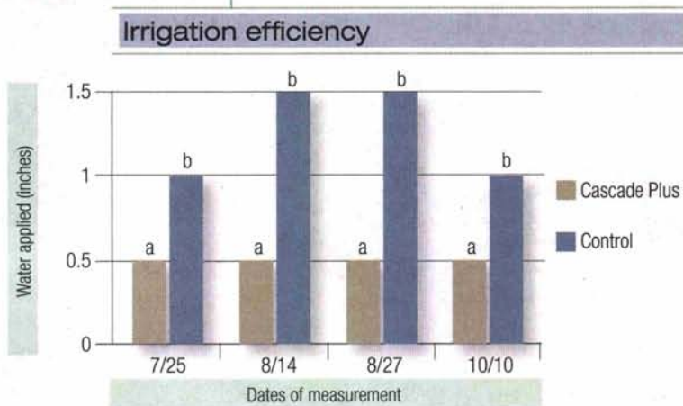
Figure 1. Amount of water required to bring soil moisture content up from 5% to 15%. Different letters at each observation date indicate a significant difference between the Cascade Plus treatment and the control.
